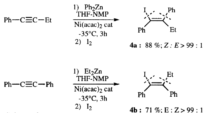
Scheme 3
