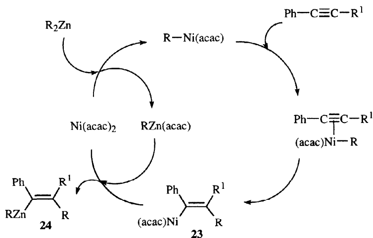
Scheme 10
