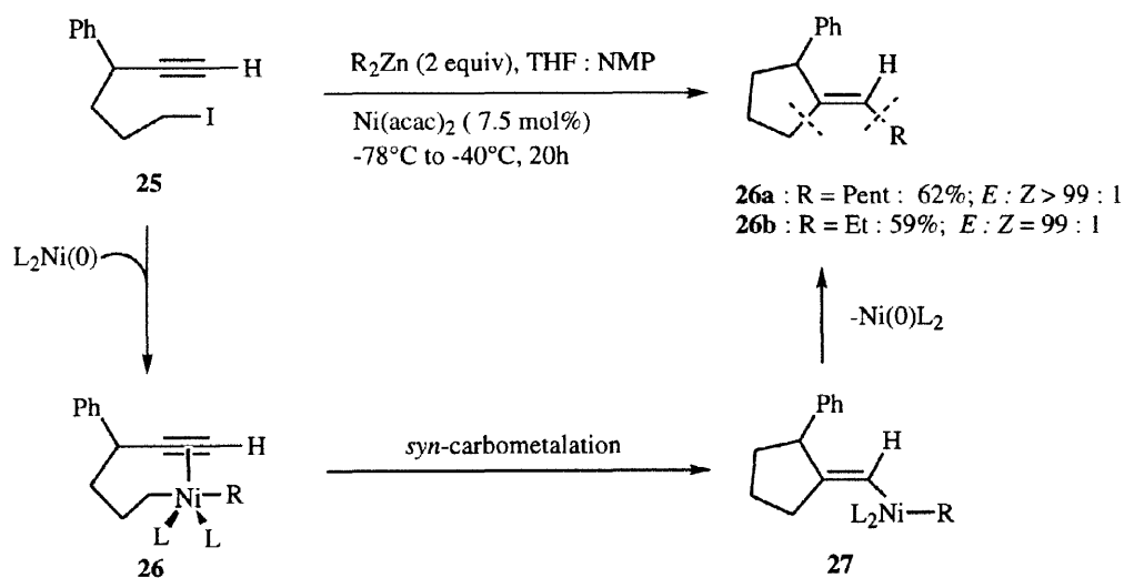
Scheme 11
